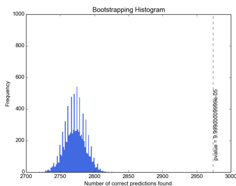
Fig. 6.5 This bootstrapping histogram shows the distribution of the number of correct predictions found when deleting a random selection of DcGO predictions (the same number as are discarded by the filter). The dotted lines shows the number of correct predictions found by the filter. The low p-value ( 9.99 \times 10^{-5} ) shows the low probability of the filter performing at least as well as it has (in terms of the number of correct predictions) by random chance.
