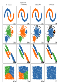
Fig. 4.8 Comparison illustrating differences between the implemented clustering methods. Image adapted from sklearn documentation[184].
