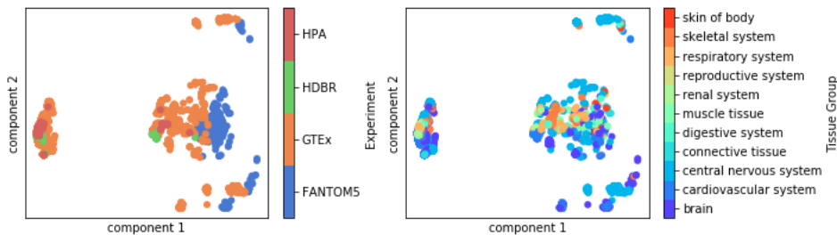
Fig. 8.10 PCA (Principal Components Analysis) plot showing batch effects present in the combined dataset.
