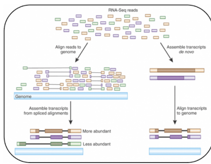
Fig. 3.2 Image showing how RNA-Seq reads are mapped to the genome (image from Advancing RNA-Seq Analysis [47]). RNA-seq is used much less often for de novo sequencing, and is generally mapped to a reference sequence.
