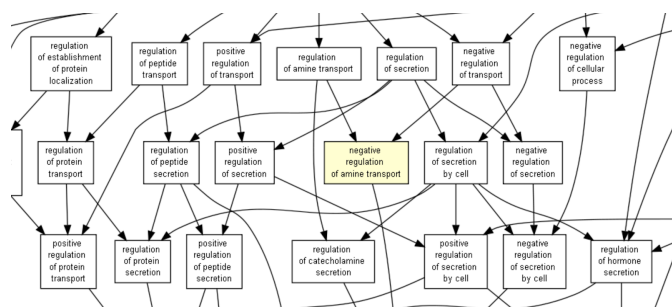
Fig. 3.4 A subsection of the Gene Ontology with arrows showing the existence of relationships (image generated using GOrilla[95])
