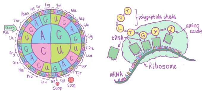
Fig. 2.4 Left: An amino acid wheel chart showing the mapping between nucleotide codons of RNA and amino acids. The chart is read from the inside out, for example UGA is a stop codon and UUG encodes for leucine “Leu”). Right: An illustration of the translation process, showing tRNAs delivering amino acids to the ribosome in order to build the polypeptide chain which makes up proteins.
