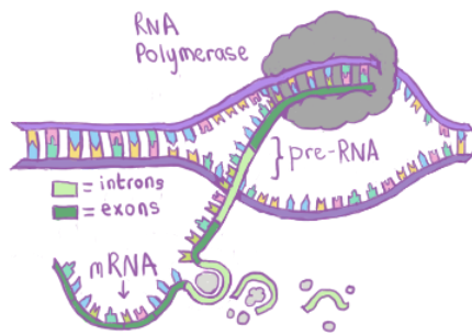
Fig. 2.3 An illustration of the transcription and splicing processes, showing the role of RNA polymerase in building RNA.
