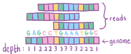
Fig. 3.1 Image illustrating how reads of DNA are aligned with one another to assemble genomes de novo .
